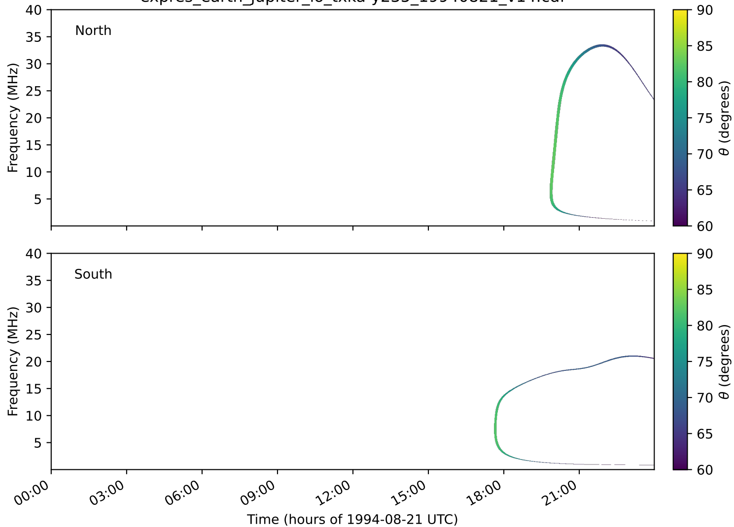
expres_earth_jupiter_io_txka-y235_19940821_v14.cdf
