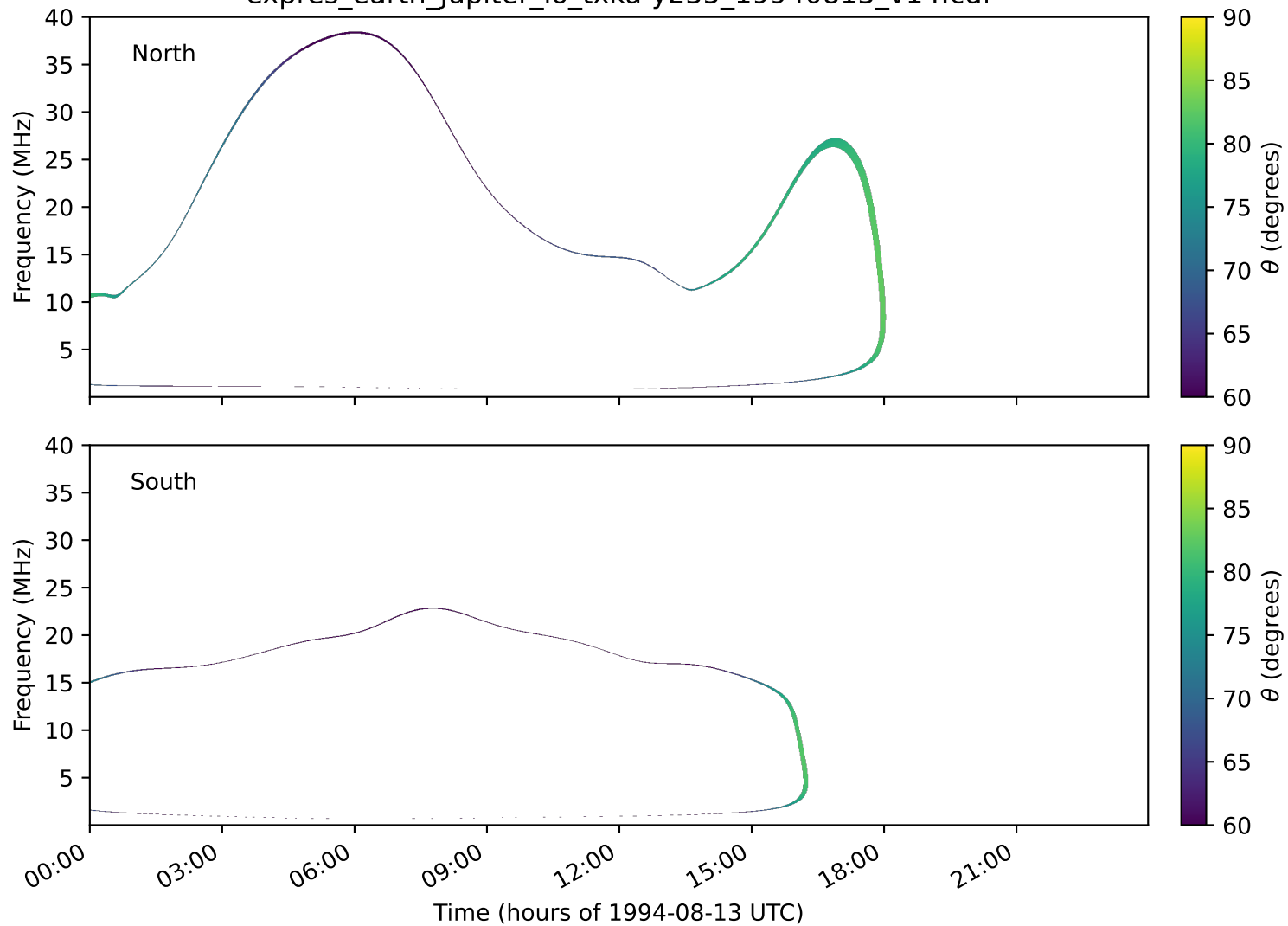
expres_earth_jupiter_io_txka-y235_19940813_v14.cdf
