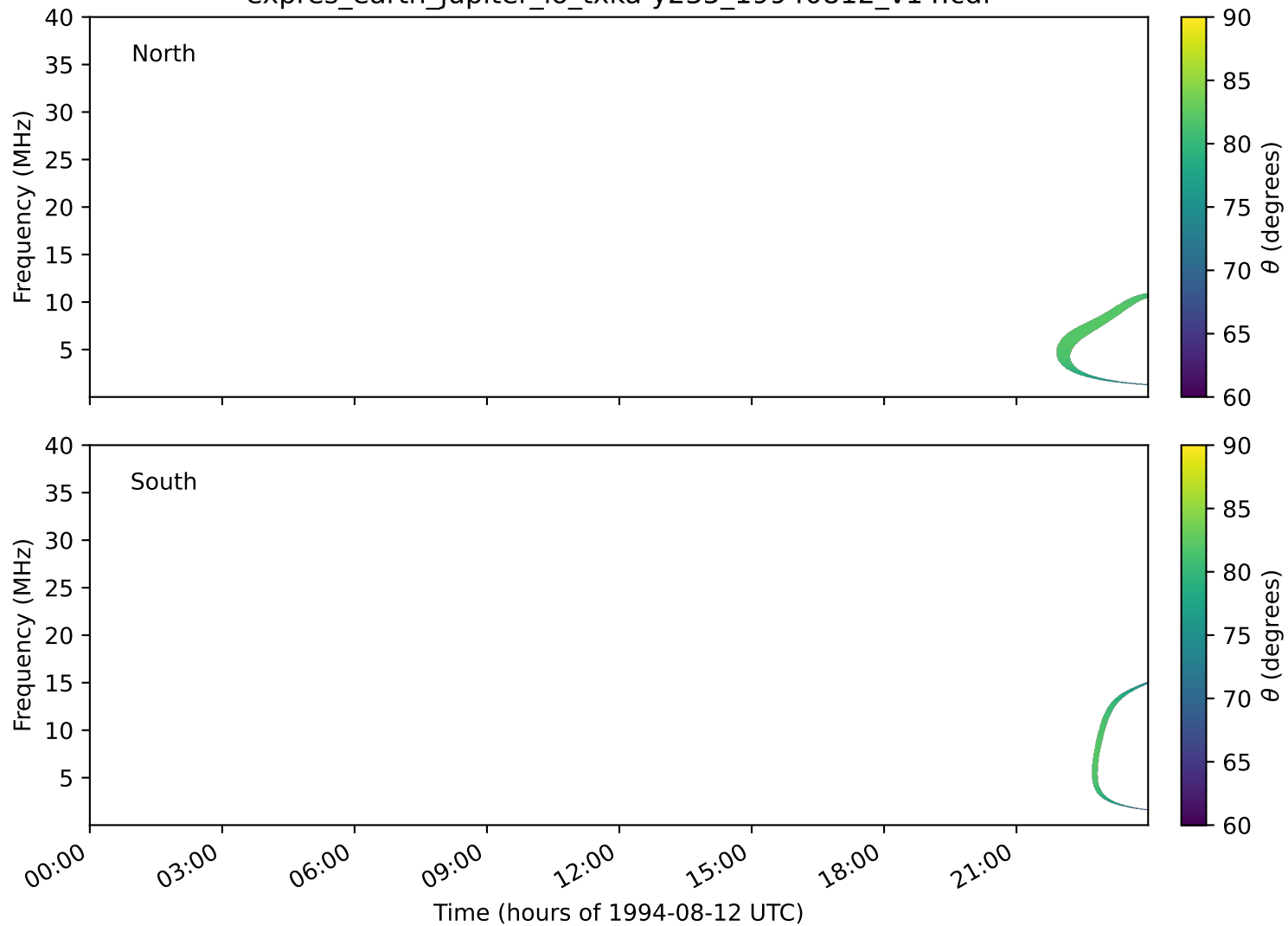
expres_earth_jupiter_io_txka-y235_19940812_v14.cdf
