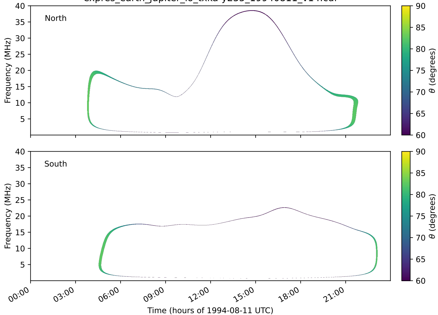
expres_earth_jupiter_io_txka-y235_19940811_v14.cdf
