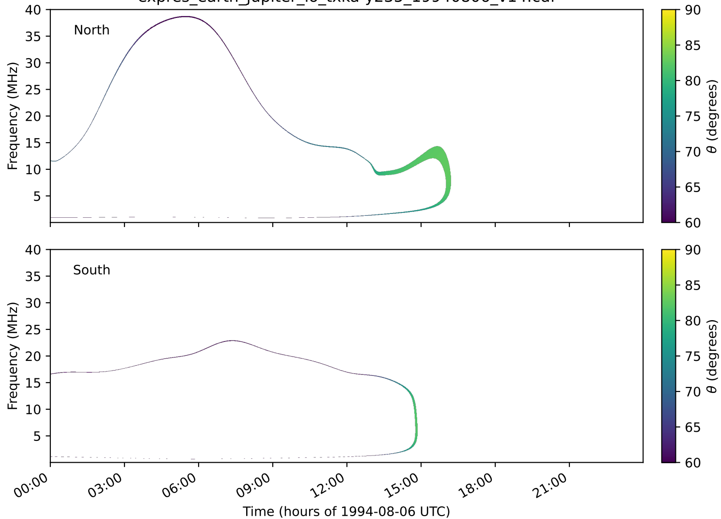
expres_earth_jupiter_io_txka-y235_19940806_v14.cdf
