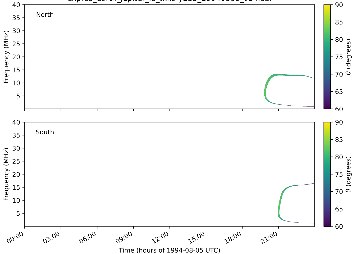
expres_earth_jupiter_io_txka-y235_19940805_v14.cdf
