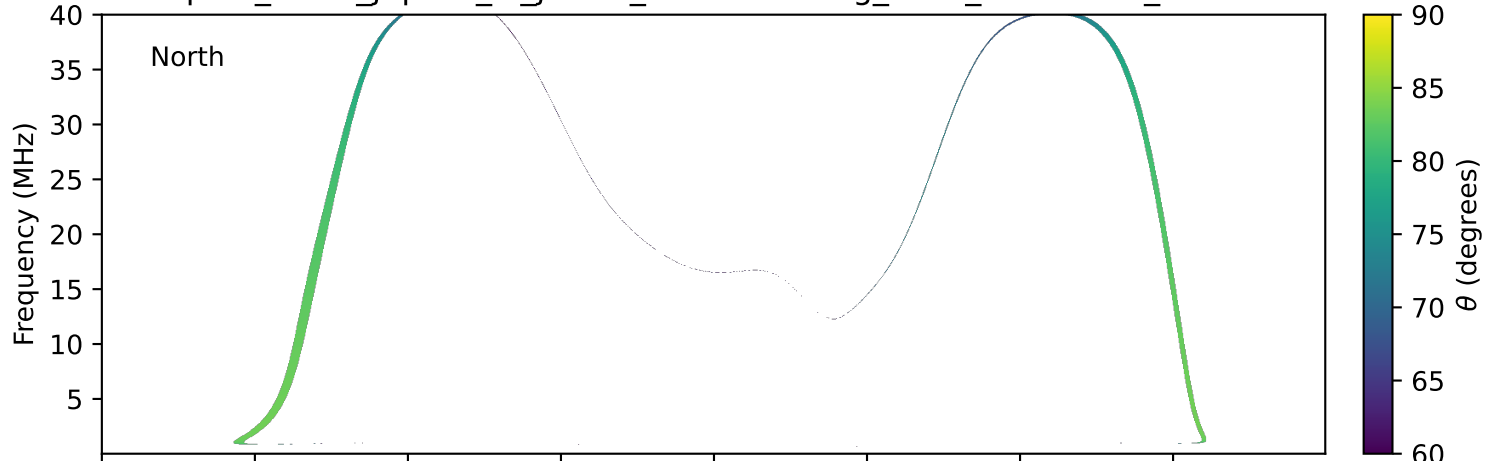
expres_earth_jupiter_io_jrm33_lossc-wid1deg_3kev_19940827_v11.cdf
