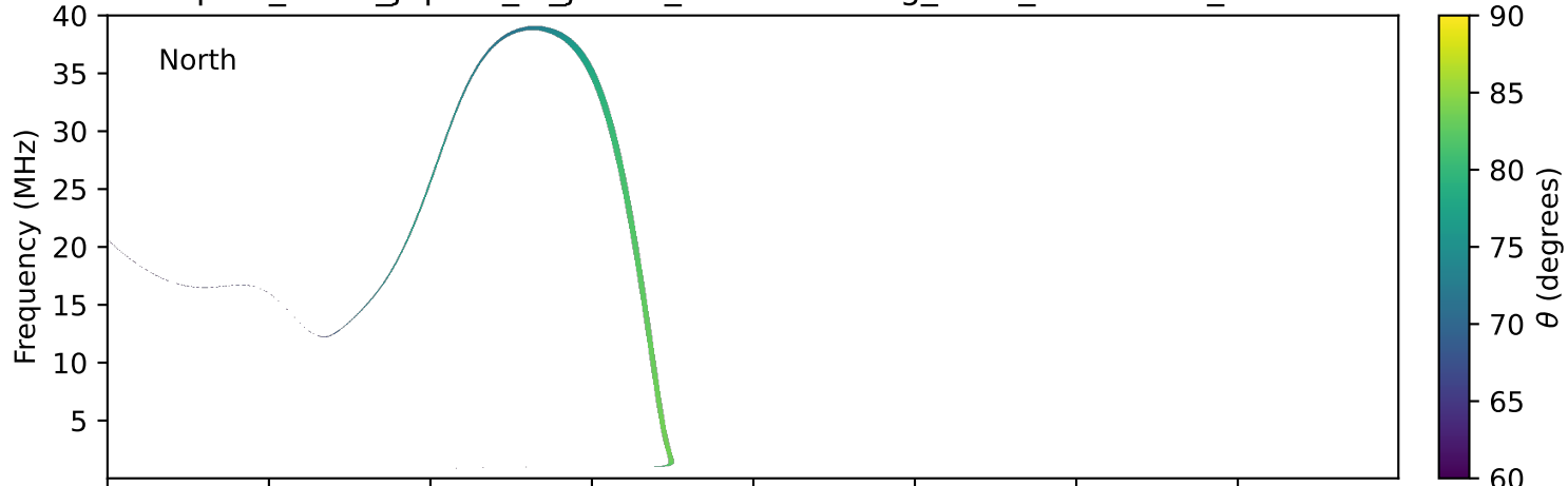
expres_earth_jupiter_io_jrm33_lossc-wid1deg_3kev_19940808_v11.cdf
