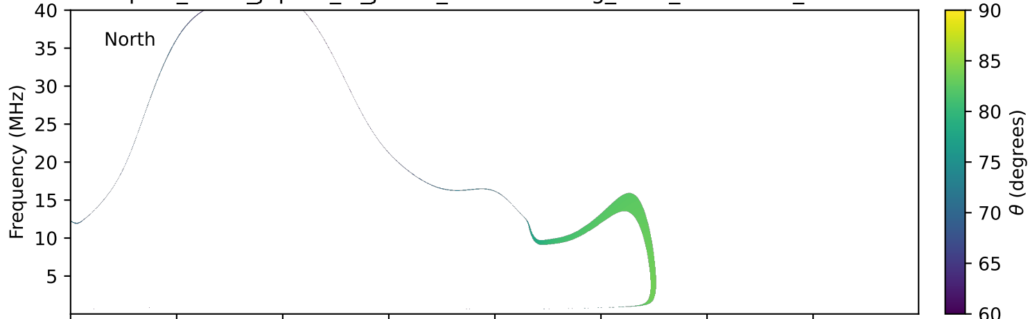
expres_earth_jupiter_io_jrm33_lossc-wid1deg_3kev_19940806_v11.cdf
