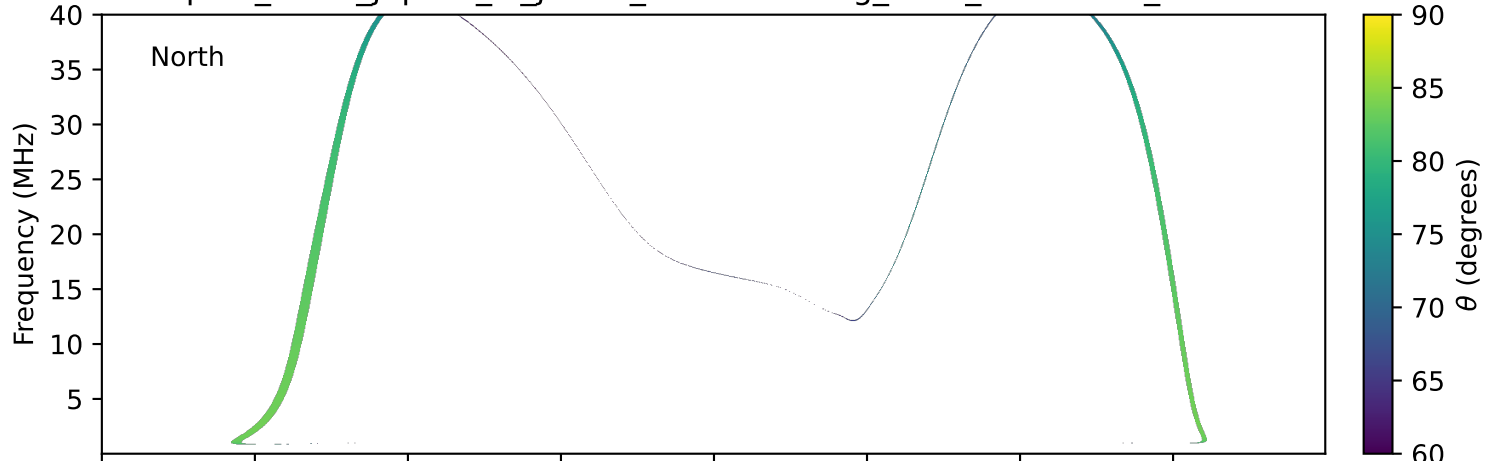
expres_earth_jupiter_io_jrm09_lossc-wid1deg_3kev_19940827_v11.cdf
