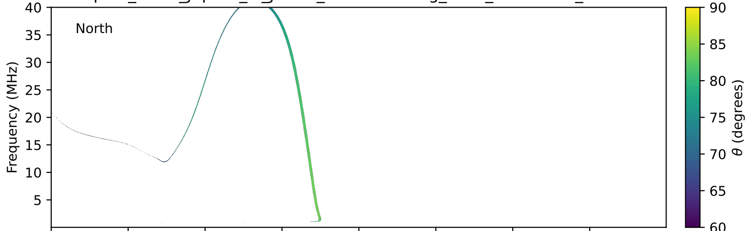
expres_earth_jupiter_io_jrm09_lossc-wid1deg_3kev_19940808_v11.cdf
