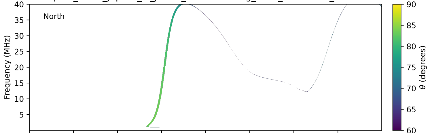
expres_earth_jupiter_io_jrm09_lossc-wid1deg_3kev_19940802_v11.cdf
