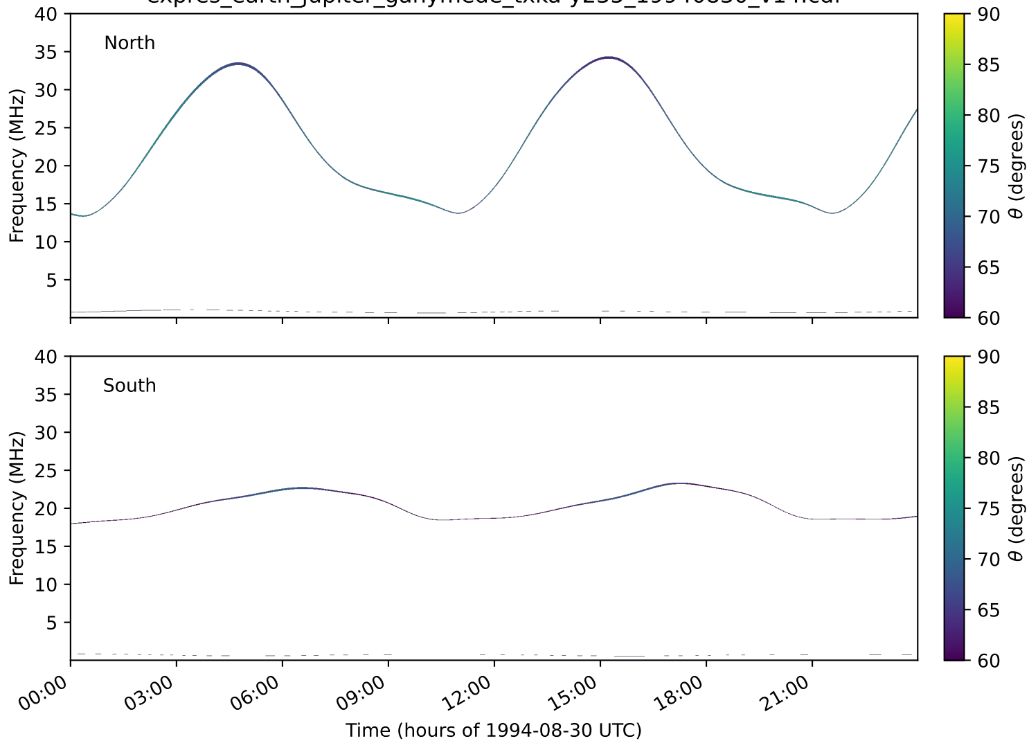
expres_earth_jupiter_ganymede_txka-y235_19940830_v14.cdf
