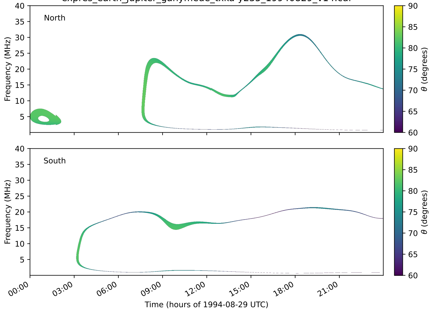
expres_earth_jupiter_ganymede_txka-y235_19940829_v14.cdf
