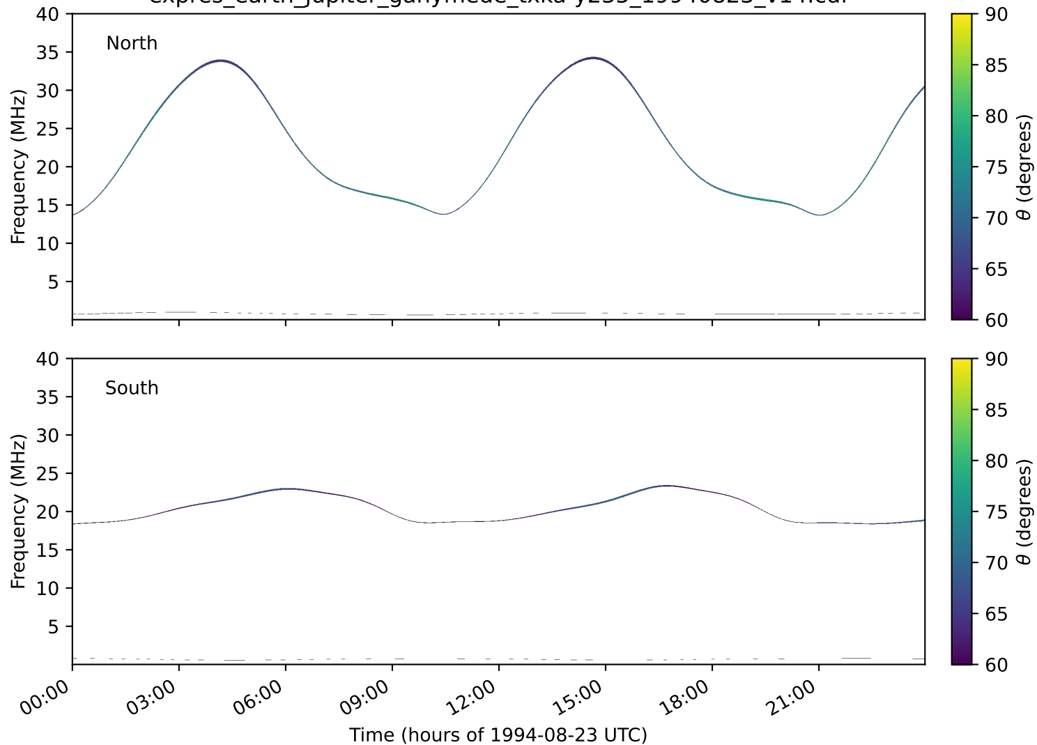
expres_earth_jupiter_ganymede_txka-y235_19940823_v14.cdf
