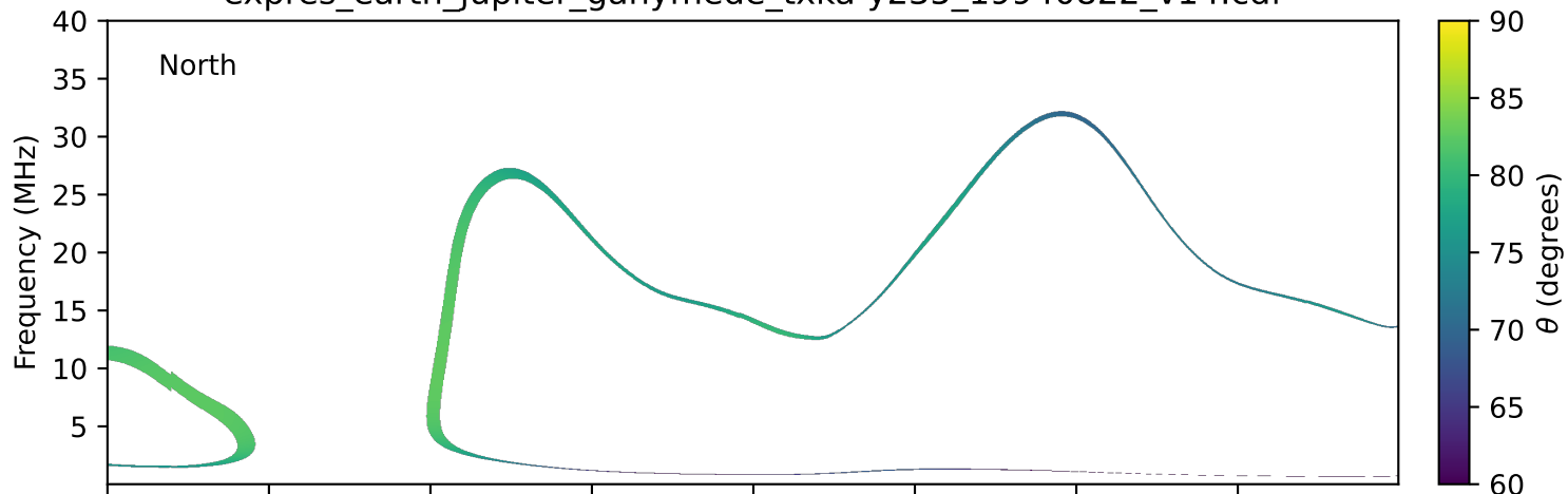
expres_earth_jupiter_ganymede_txka-y235_19940822_v14.cdf
