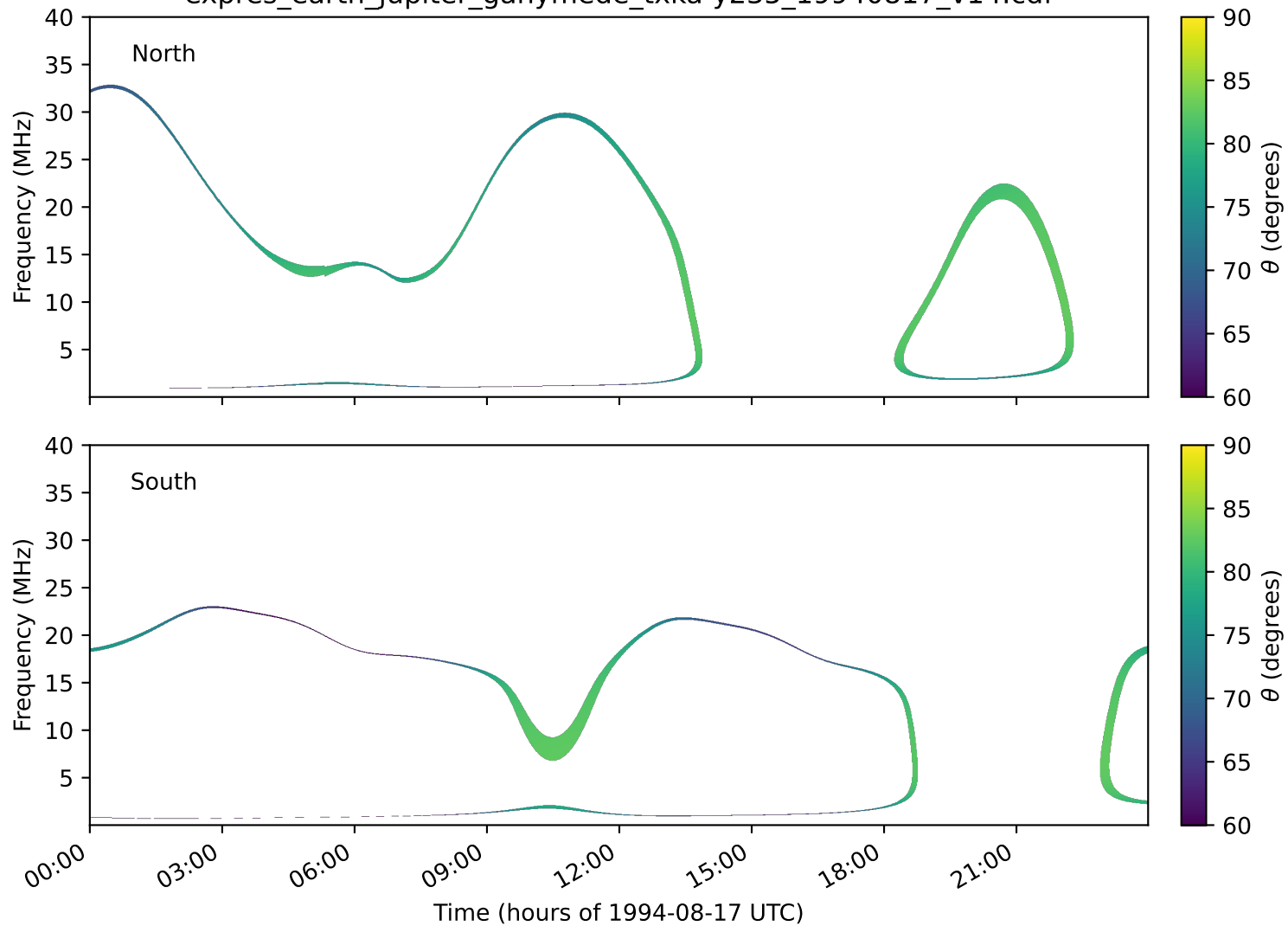
expres_earth_jupiter_ganymede_txka-y235_19940817_v14.cdf
