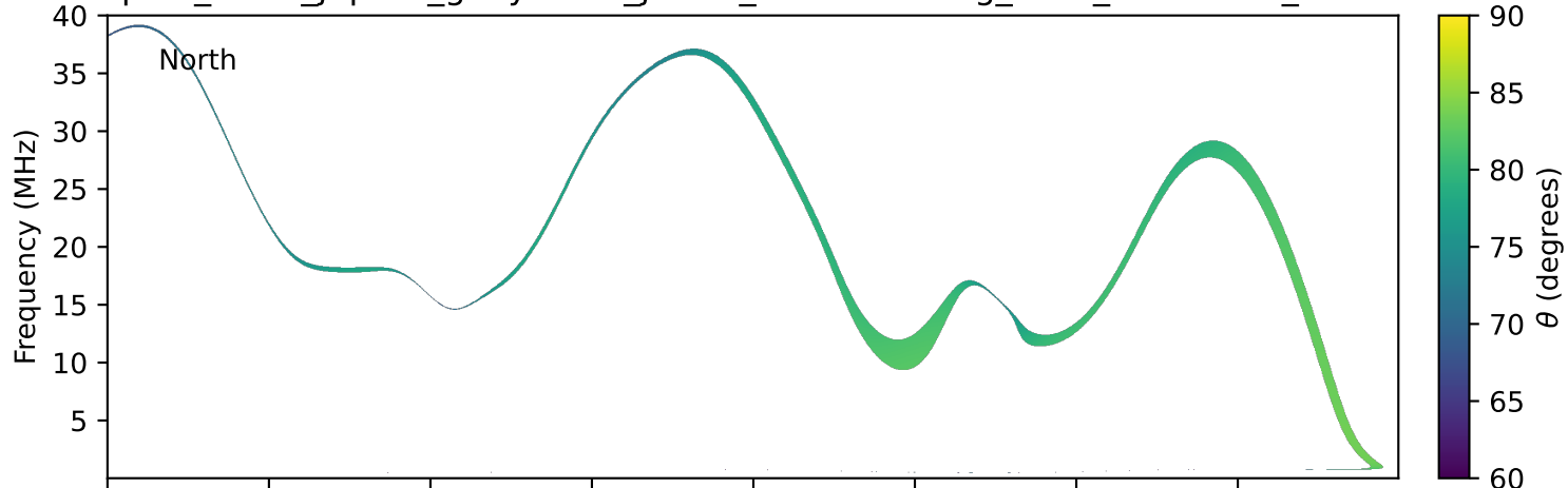
expres_earth_jupiter_ganymede_jrm33_lossc-wid1deg_3kev_19940817_v11.cdf
