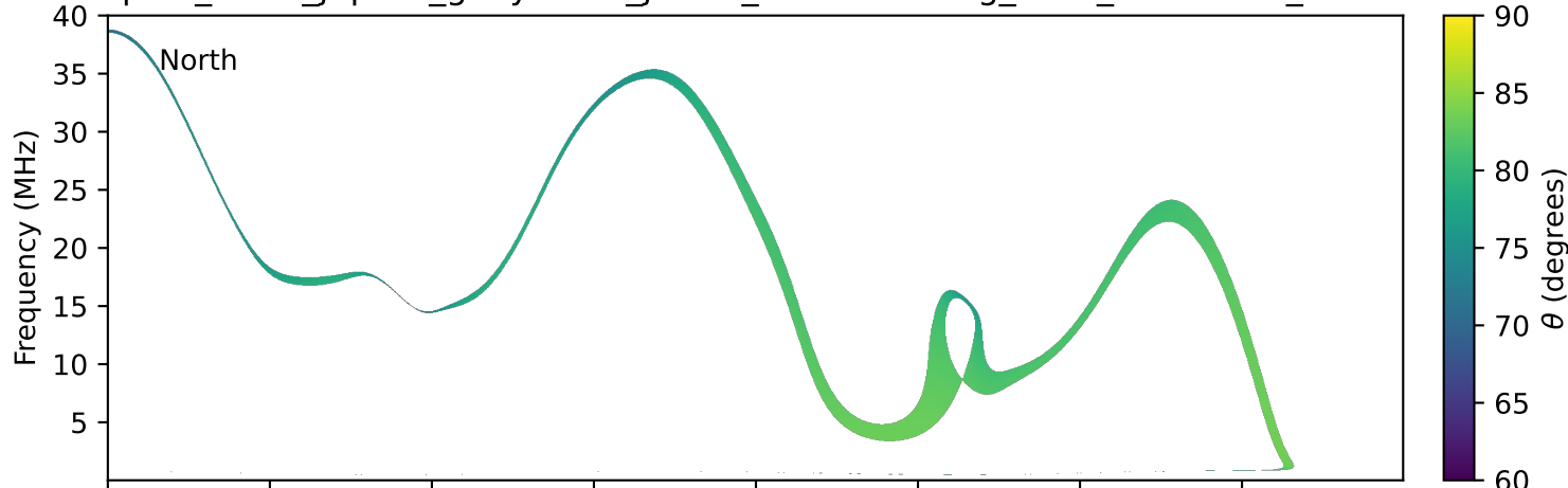
expres_earth_jupiter_ganymede_jrm33_lossc-wid1deg_3kev_19940810_v11.cdf
