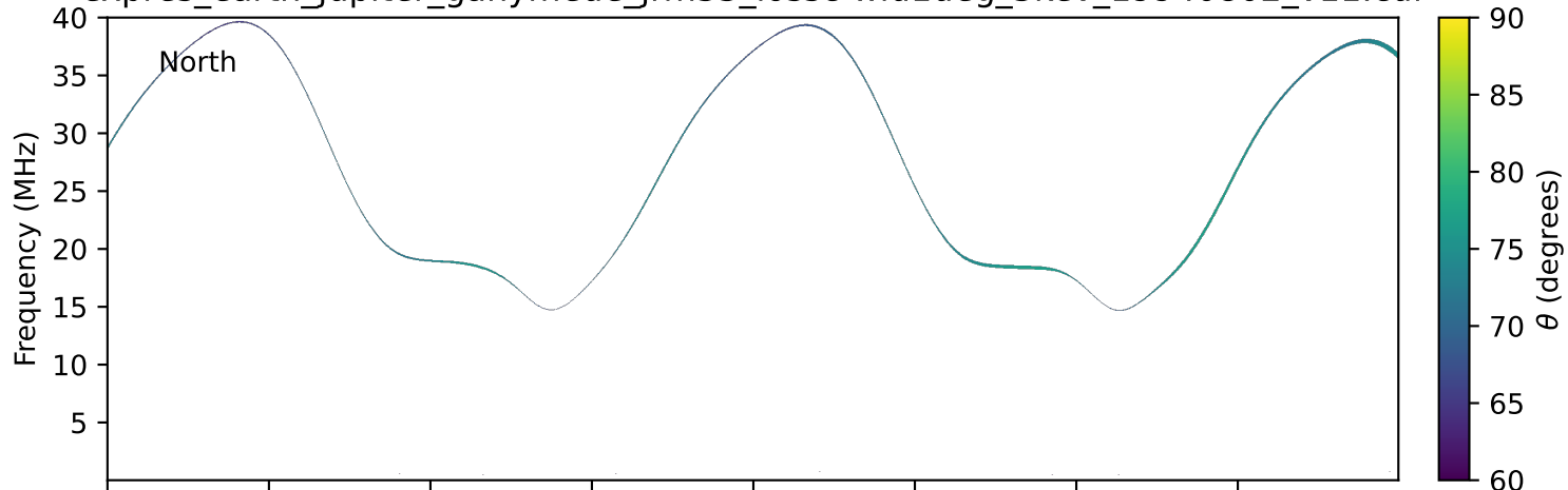
expres_earth_jupiter_ganymede_jrm33_lossc-wid1deg_3kev_19940802_v11.cdf
