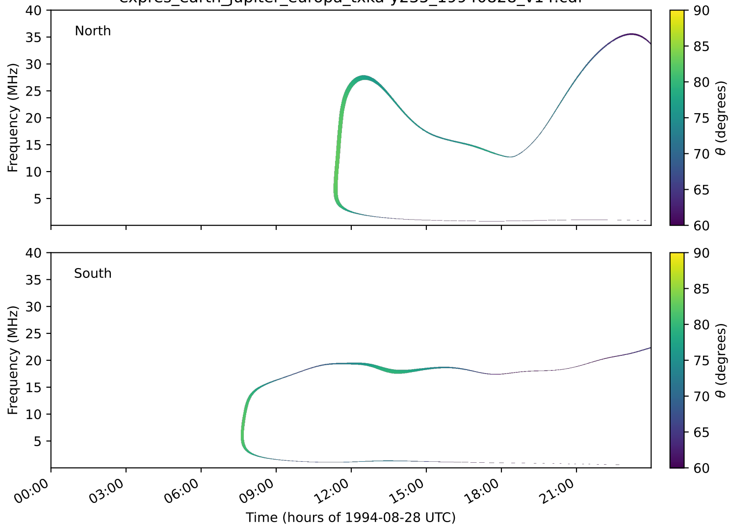
expres_earth_jupiter_europa_txka-y235_19940828_v14.cdf
