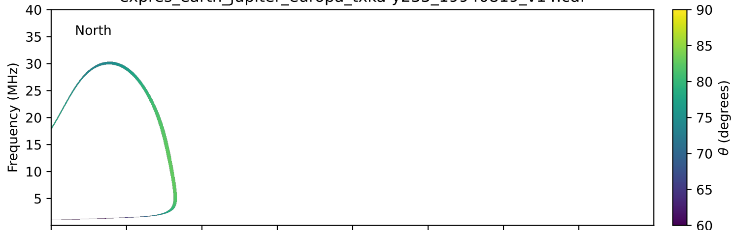
expres_earth_jupiter_europa_txka-y235_19940819_v14.cdf
