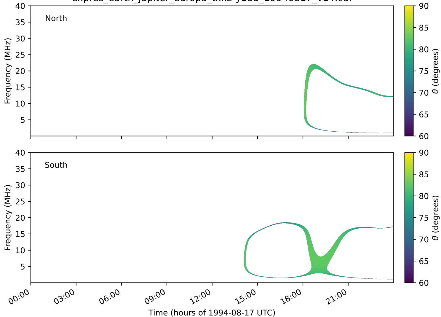
expres_earth_jupiter_europa_txka-y235_19940817_v14.cdf
