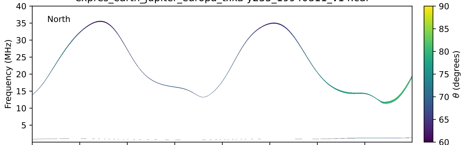
expres_earth_jupiter_europa_txka-y235_19940811_v14.cdf
