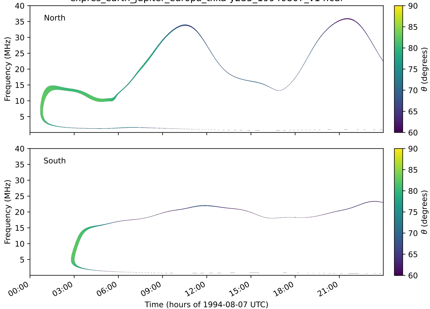
expres_earth_jupiter_europa_txka-y235_19940807_v14.cdf
