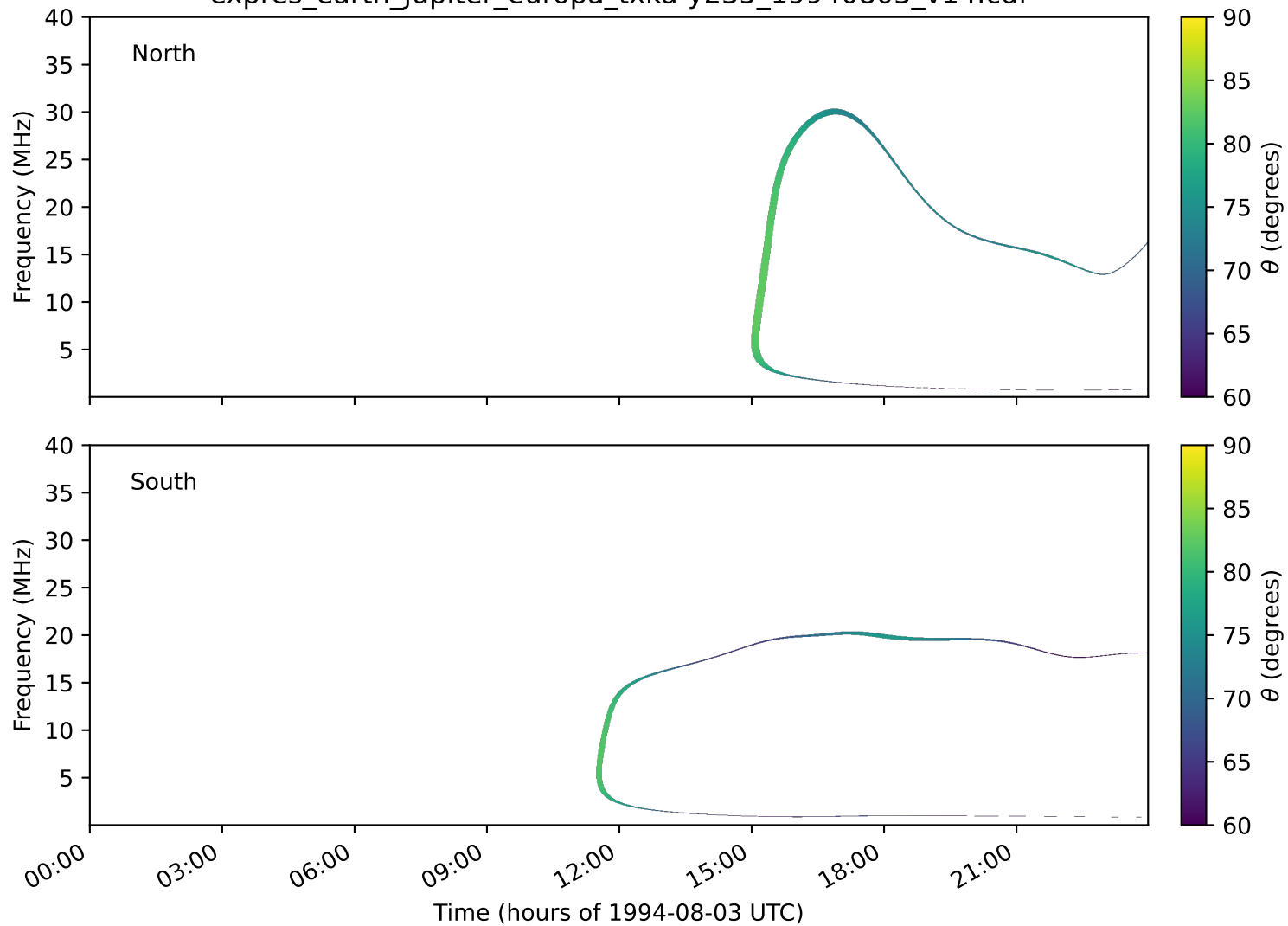
expres_earth_jupiter_europa_txka-y235_19940803_v14.cdf
