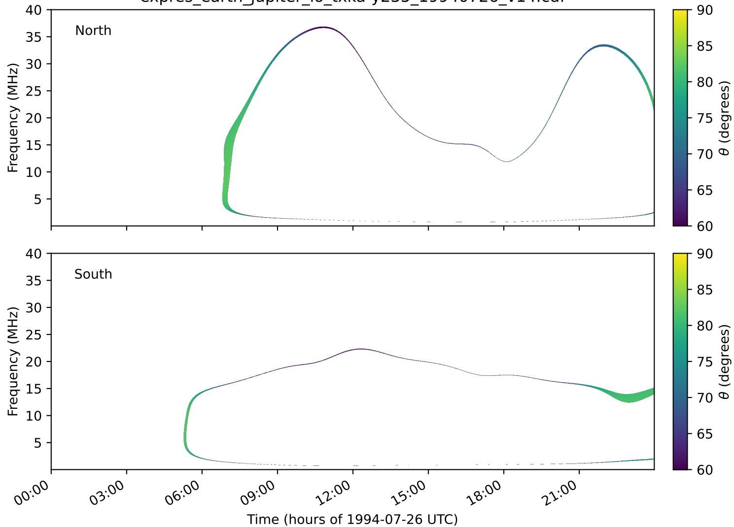
expres_earth_jupiter_io_txka-y235_19940726_v14.cdf
