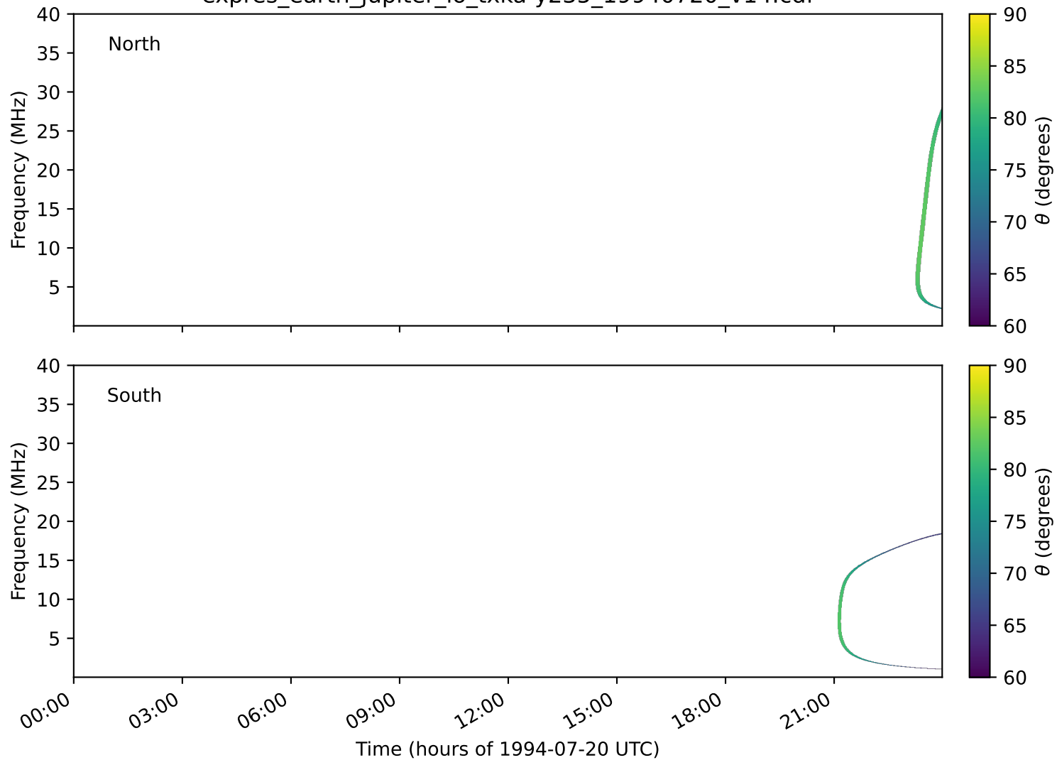
expres_earth_jupiter_io_txka-y235_19940720_v14.cdf
