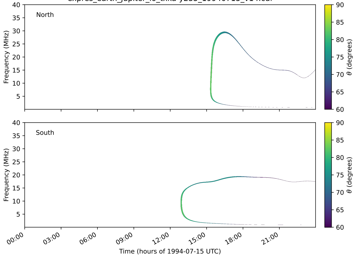
expres_earth_jupiter_io_txka-y235_19940715_v14.cdf
