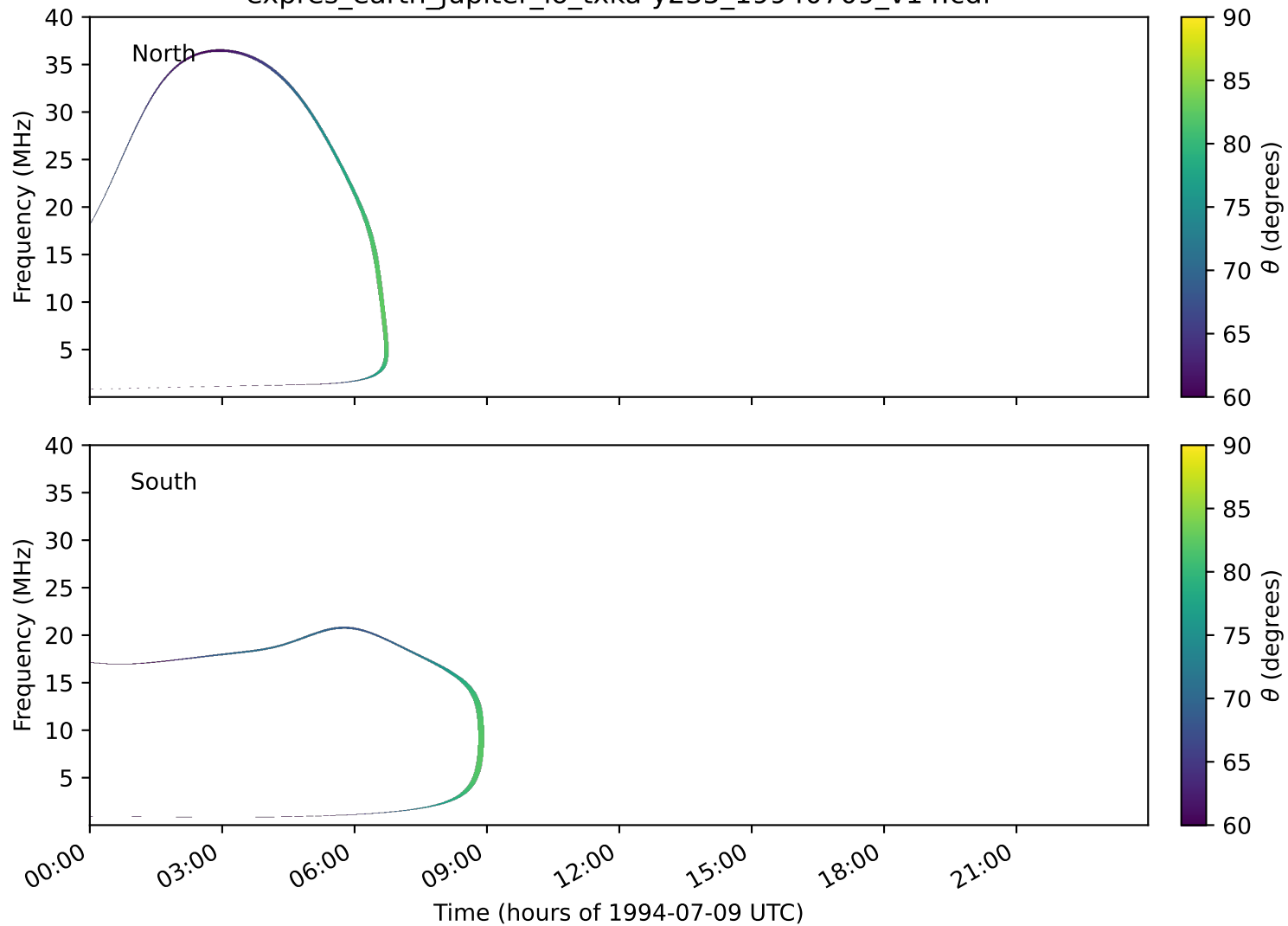
expres_earth_jupiter_io_txka-y235_19940709_v14.cdf
