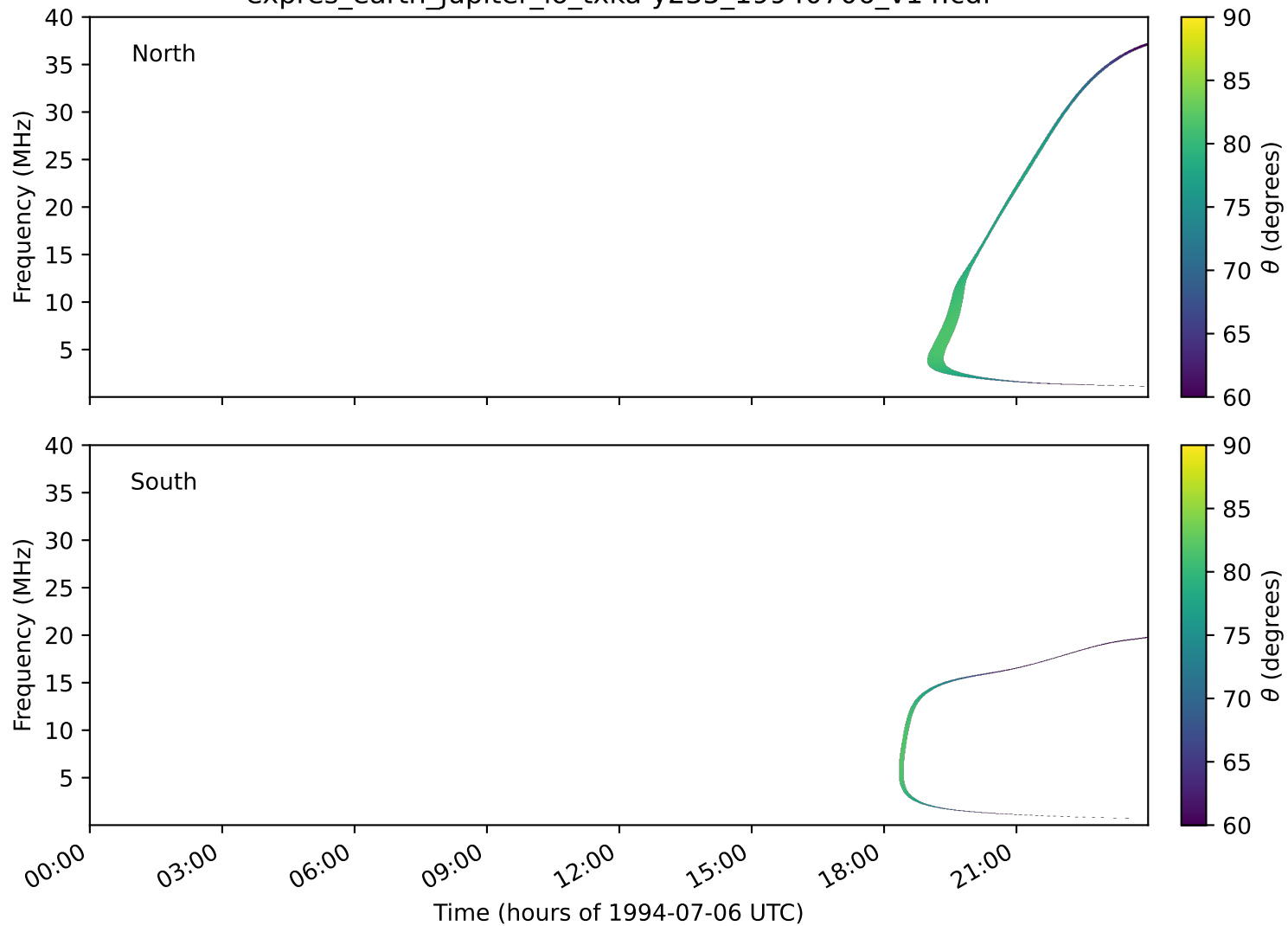
expres_earth_jupiter_io_txka-y235_19940706_v14.cdf
