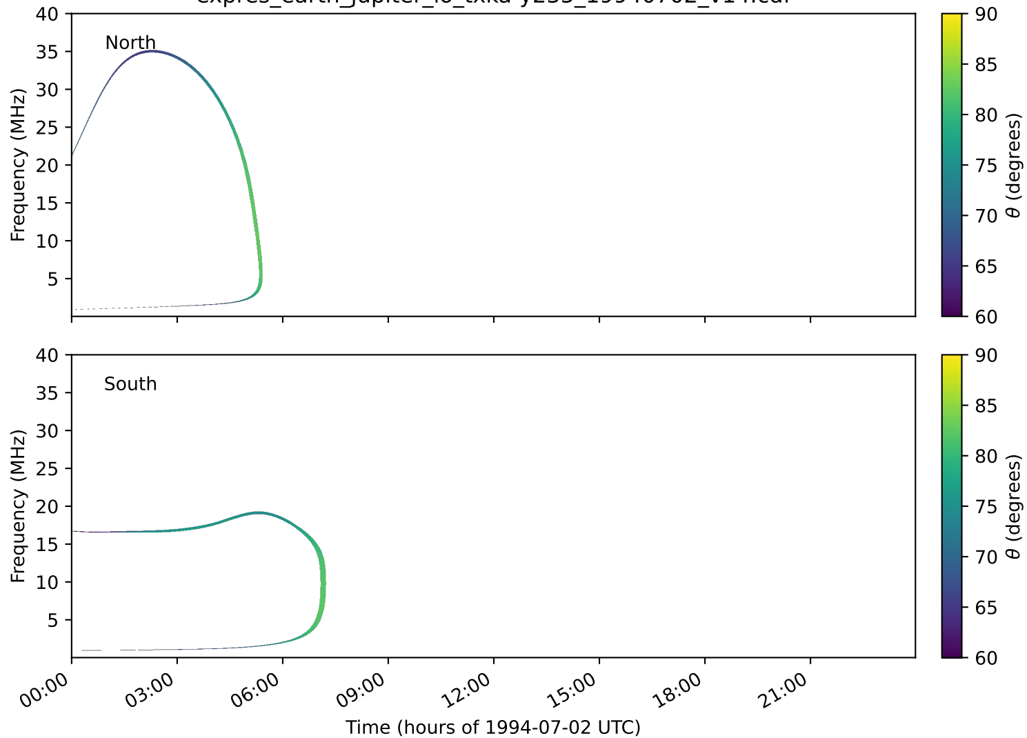
expres_earth_jupiter_io_txka-y235_19940702_v14.cdf
