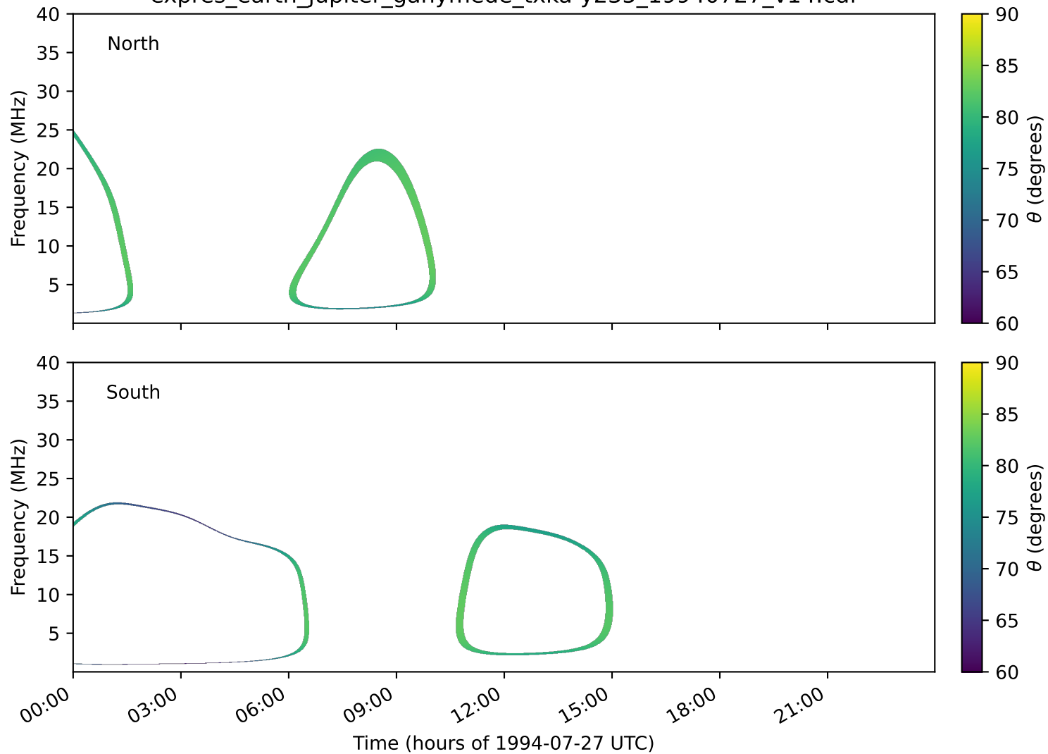
expres_earth_jupiter_ganymede_txka-y235_19940727_v14.cdf
