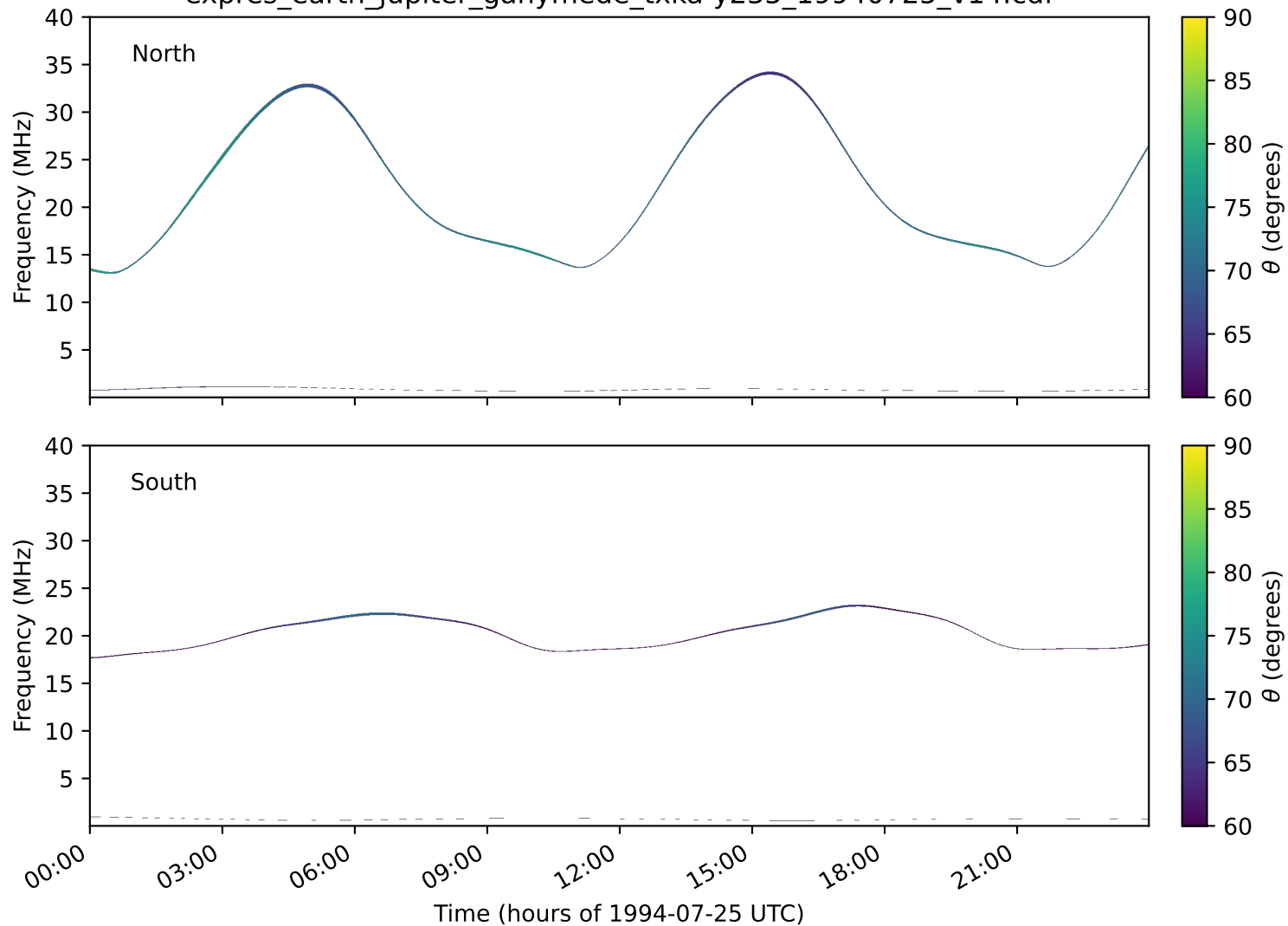
expres_earth_jupiter_ganymede_txka-y235_19940725_v14.cdf
