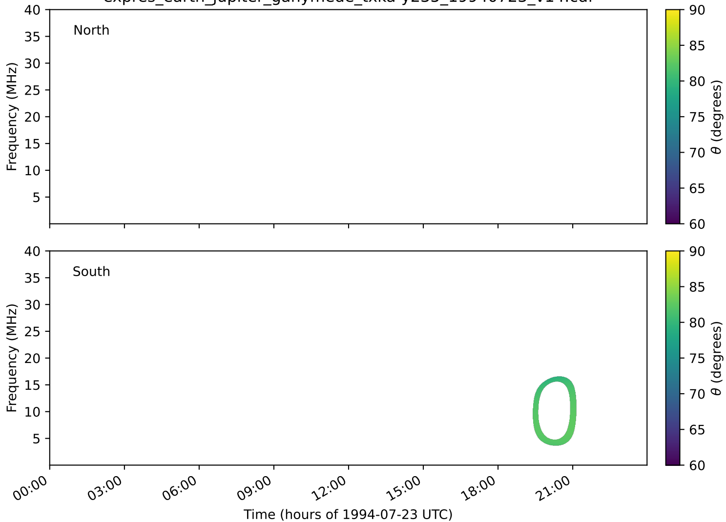
expres_earth_jupiter_ganymede_txka-y235_19940723_v14.cdf
