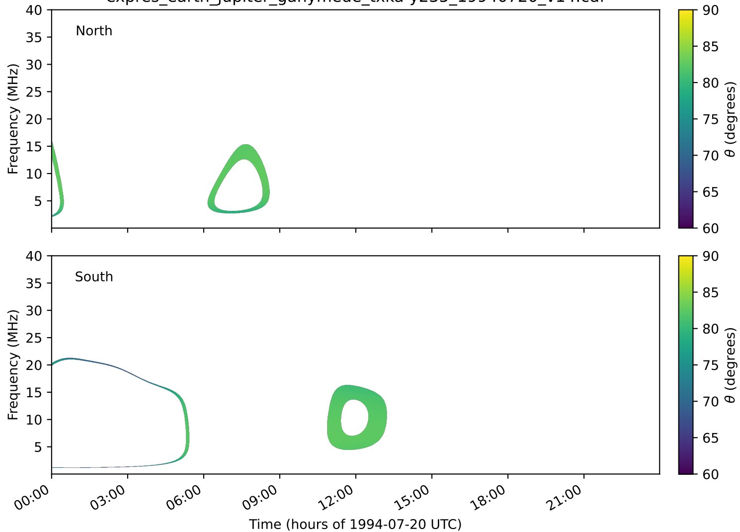
expres_earth_jupiter_ganymede_txka-y235_19940720_v14.cdf
