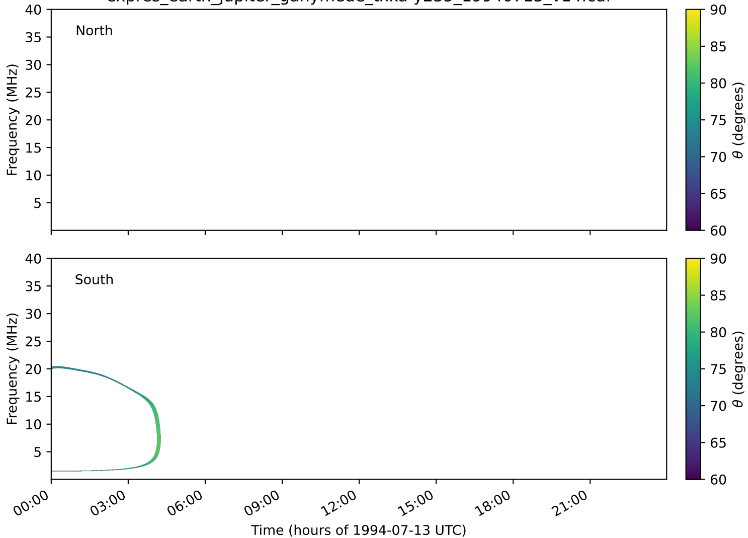
expres_earth_jupiter_ganymede_txka-y235_19940713_v14.cdf
