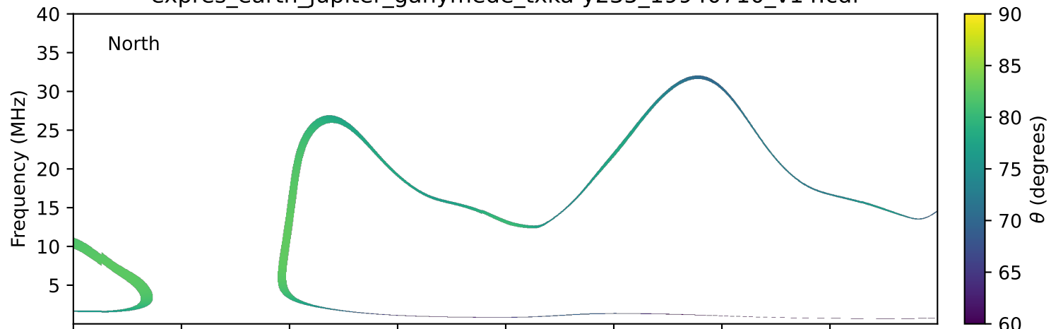
expres_earth_jupiter_ganymede_txka-y235_19940710_v14.cdf
