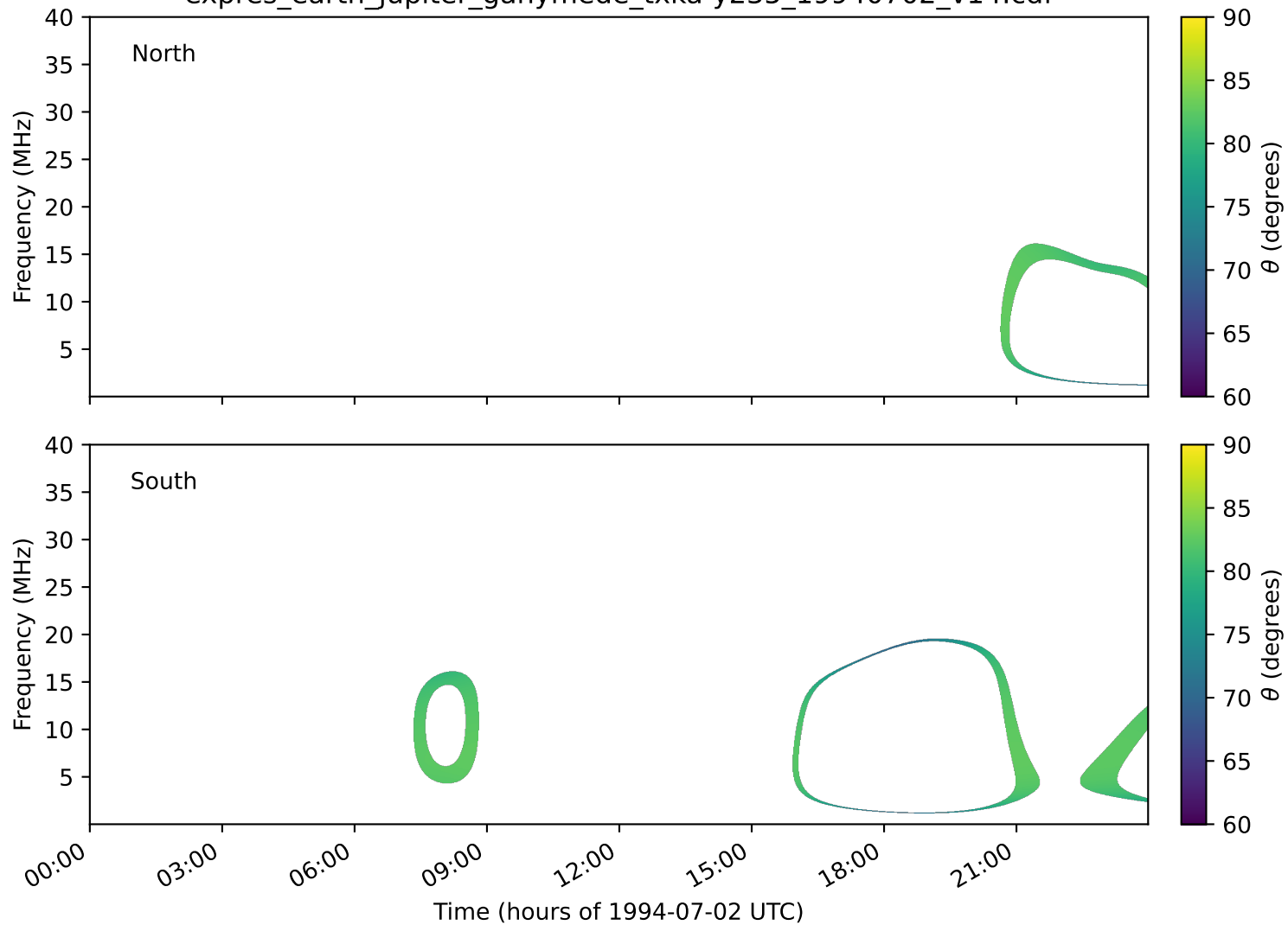
expres_earth_jupiter_ganymede_txka-y235_19940702_v14.cdf
