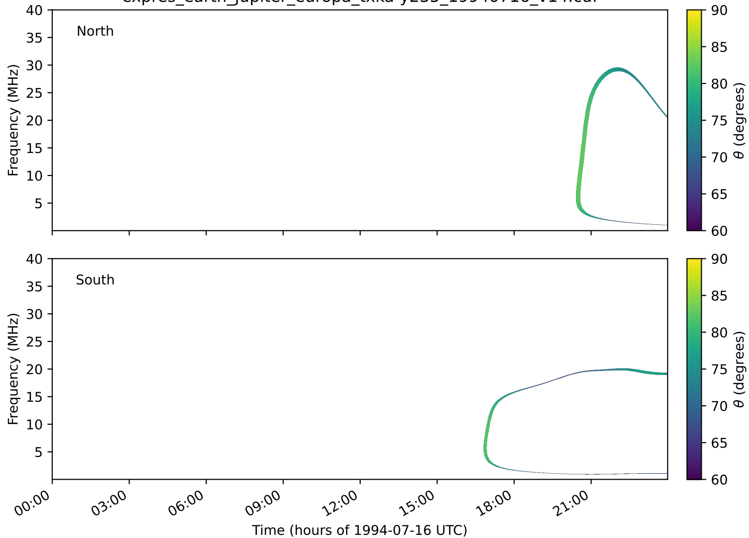
expres_earth_jupiter_europa_txka-y235_19940716_v14.cdf
