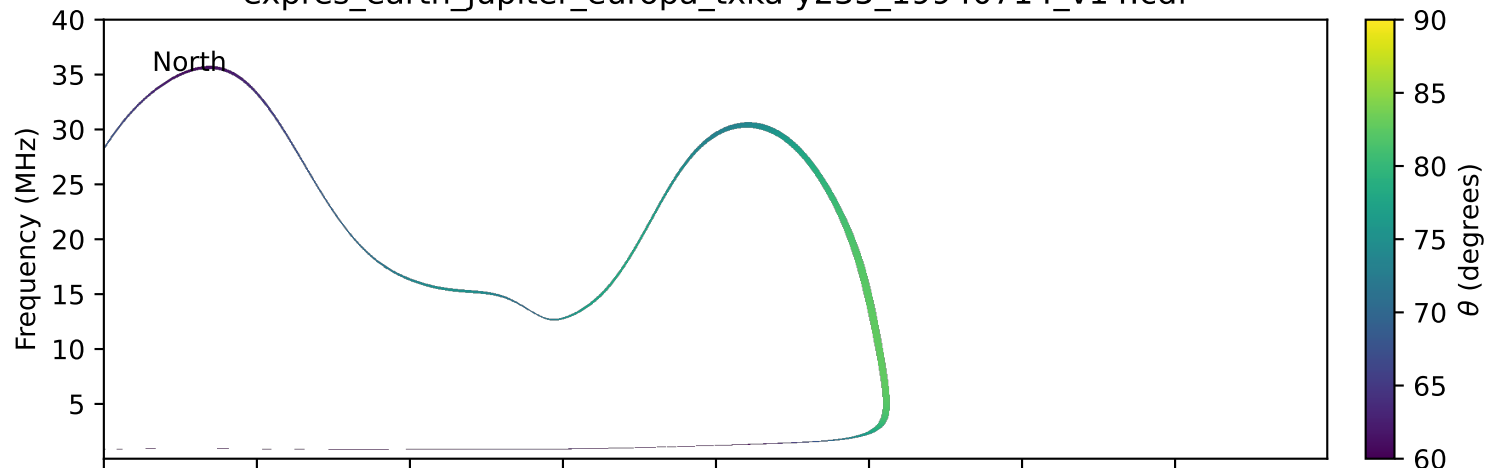
expres_earth_jupiter_europa_txka-y235_19940714_v14.cdf
