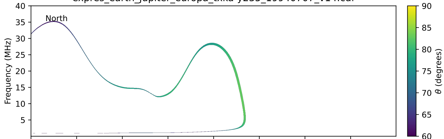
expres_earth_jupiter_europa_txka-y235_19940707_v14.cdf
