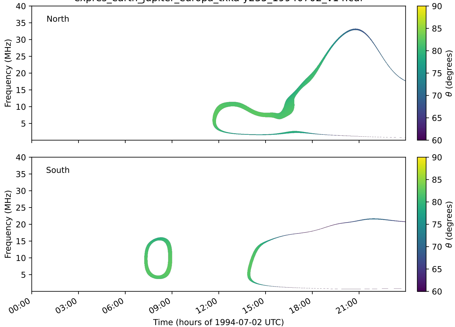
expres_earth_jupiter_europa_txka-y235_19940702_v14.cdf
