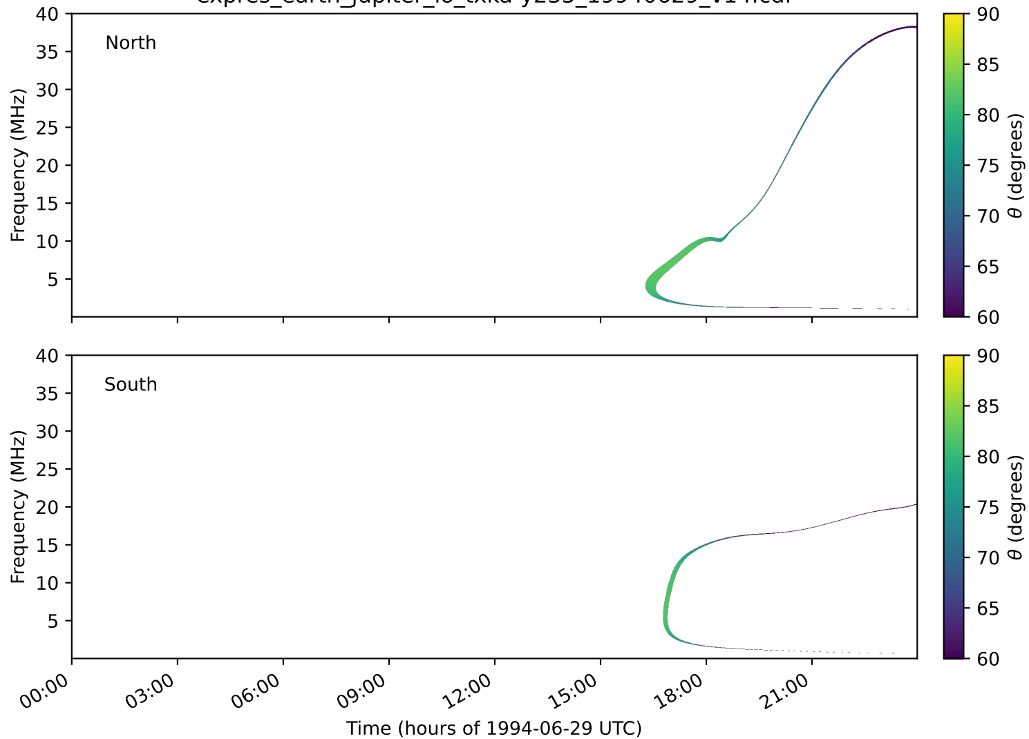
expres_earth_jupiter_io_txka-y235_19940629_v14.cdf
