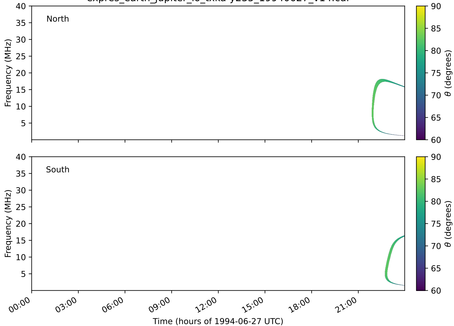
expres_earth_jupiter_io_txka-y235_19940627_v14.cdf
