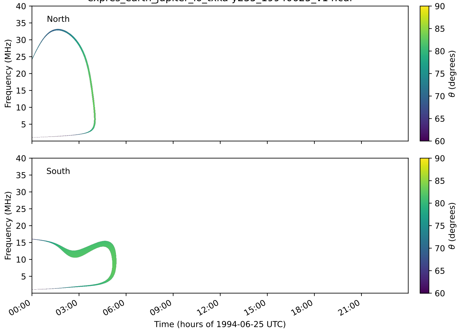
expres_earth_jupiter_io_txka-y235_19940625_v14.cdf
