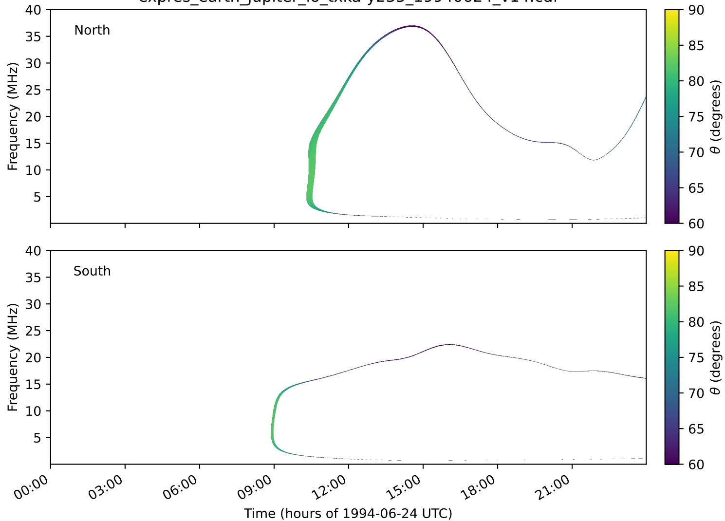
expres_earth_jupiter_io_txka-y235_19940624_v14.cdf
