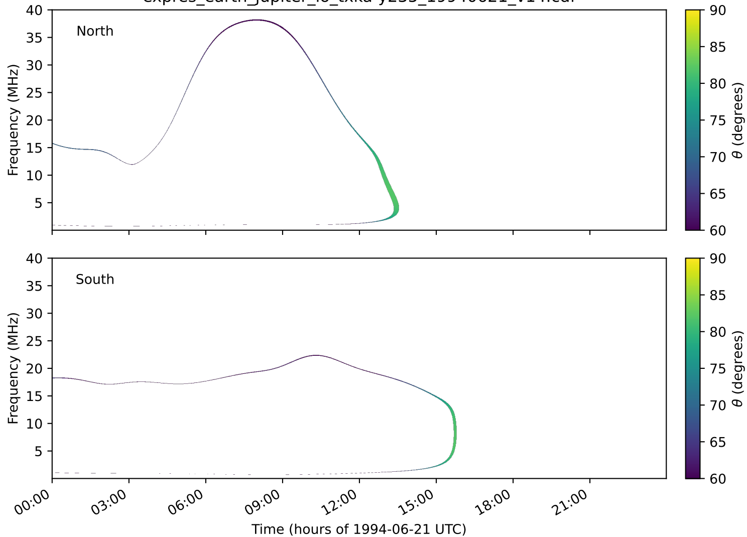
expres_earth_jupiter_io_txka-y235_19940621_v14.cdf
