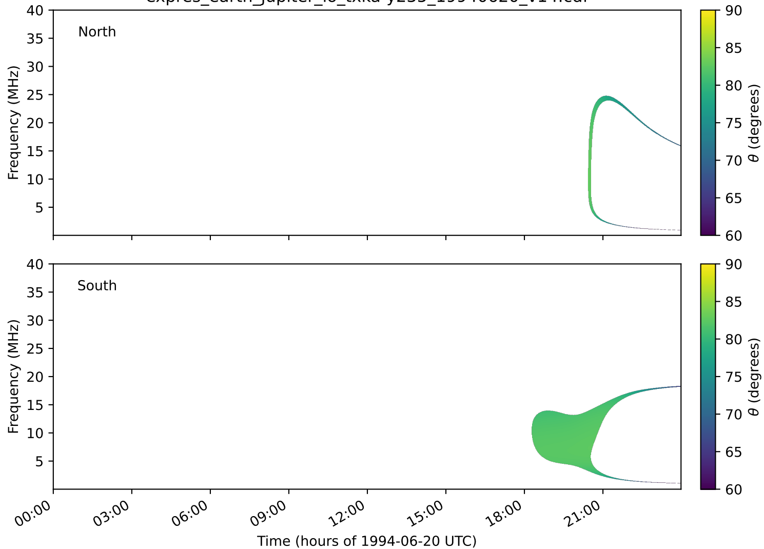
expres_earth_jupiter_io_txka-y235_19940620_v14.cdf
