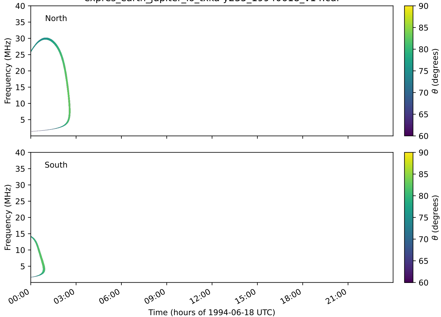
expres_earth_jupiter_io_txka-y235_19940618_v14.cdf
